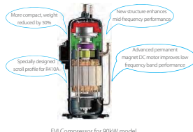
EVI Compressor for 90kW model
