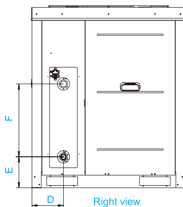
Right view MC-SU30-RN1L / MC-SU60-RN1L
