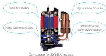
Compressor for 30/60kW models
