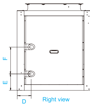
Right view MC-SU90-RN1L
